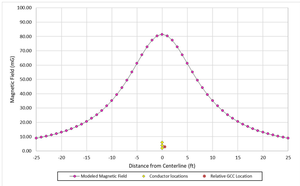
Figure 3.5 Magnetic Field Modeling Results for Direct-Buried Conduits in Vertical Configuration
