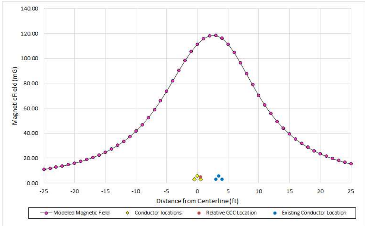
Figure 3.7 Magnetic Field Modeling Results for the Typical Direct-Buried Conduits in Trefoil Configuration in Proximity to the Existing 69-886 Southampton to Bridgehampton Underground Transmission Line
