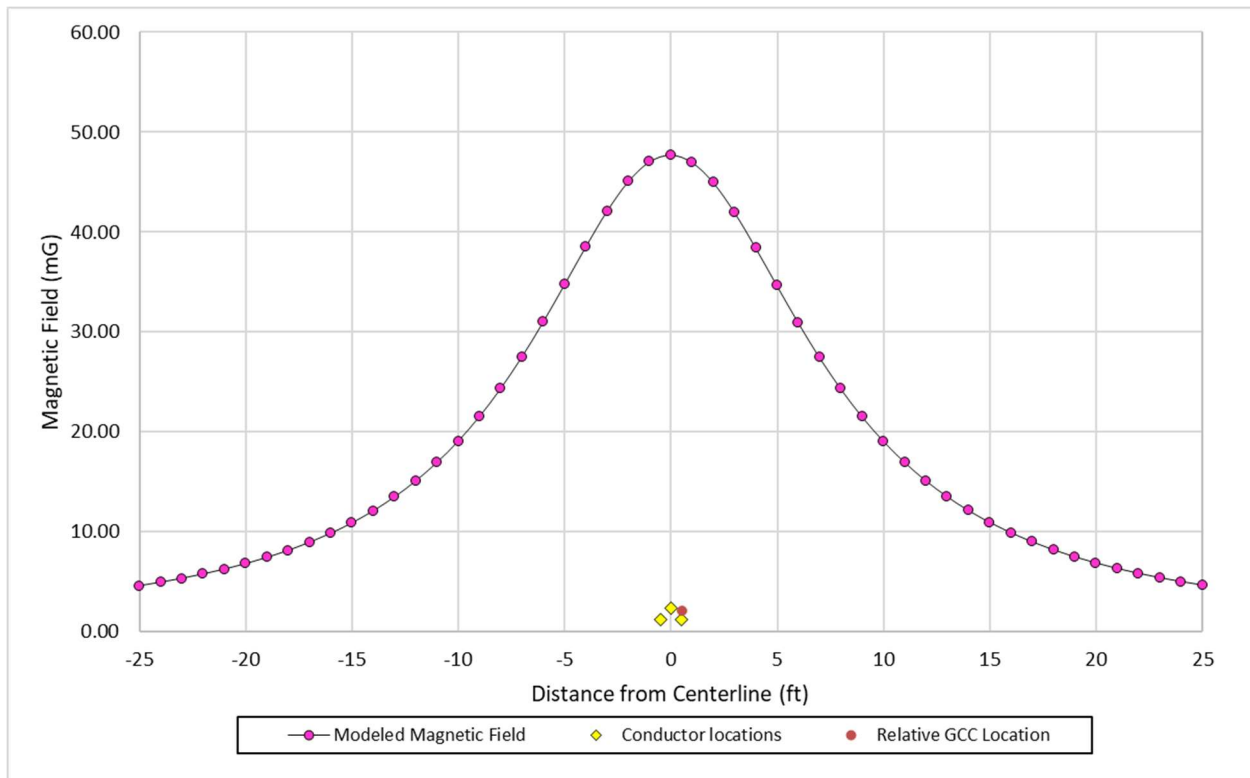
Figure 3.2 Magnetic Field Modeling Results for Typical Direct-Buried Conduits in Trefoil Configuration
